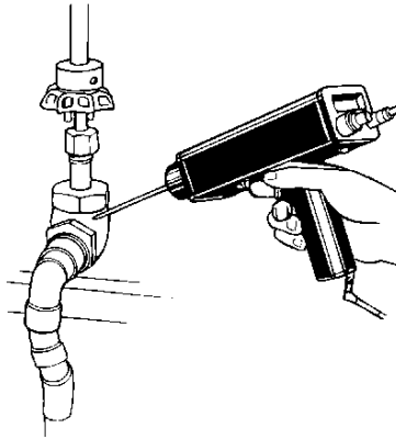
CHECKING VALVE LEAKAGE/ BLOCKAGE WITH THE ULTRAPROBE
